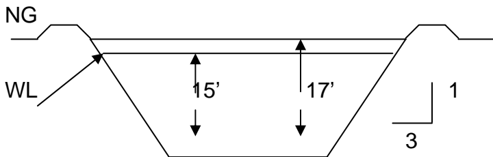
Side View Standard cross-section
