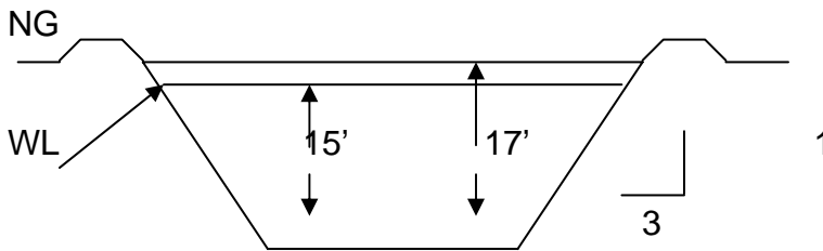
Side View Standard cross-section
