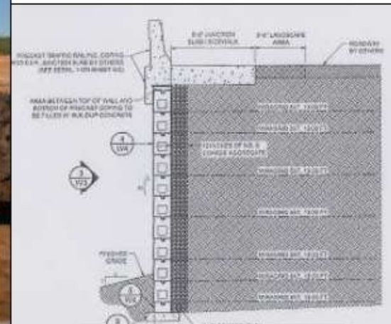
Typical Cross-Section
